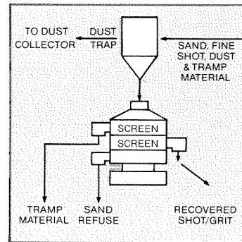
Shot and/or Grit Recovery
